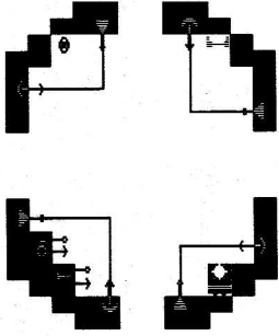
Counter-clockwise Wall-follower
