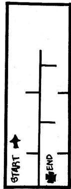
MAZE 1
